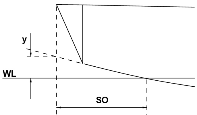
COUNTER STERN
