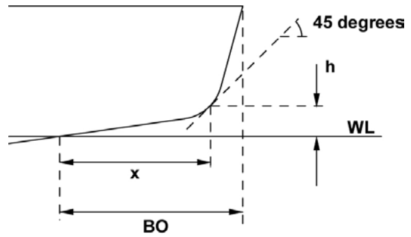
SCOW BOW OR KNUCKLE EXPOSED
