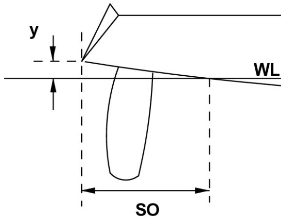
SPADE RUDDER
